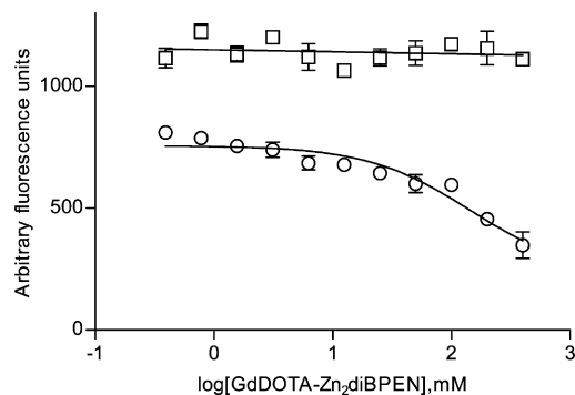
Figure 4. Displacement fluorescence plots for warfarin (squares, 5 \mu\text{M} ) and dansylglycine (circles, 5 \mu\text{M} ) from equimolar HSA by GdDOTA- \text{Zn}_2\text{diBPEN} at 25 ^\circ\text{C} in 100 mM Tris buffer at pH 7.6. The solid curves represent the best fit to the data.
